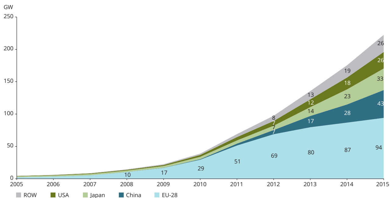
Figure 3.2 Growth in total solar PV capacity (GW) in the EU-28, the top three non-EU countries and the rest of the world (ROW), 2005-2015
