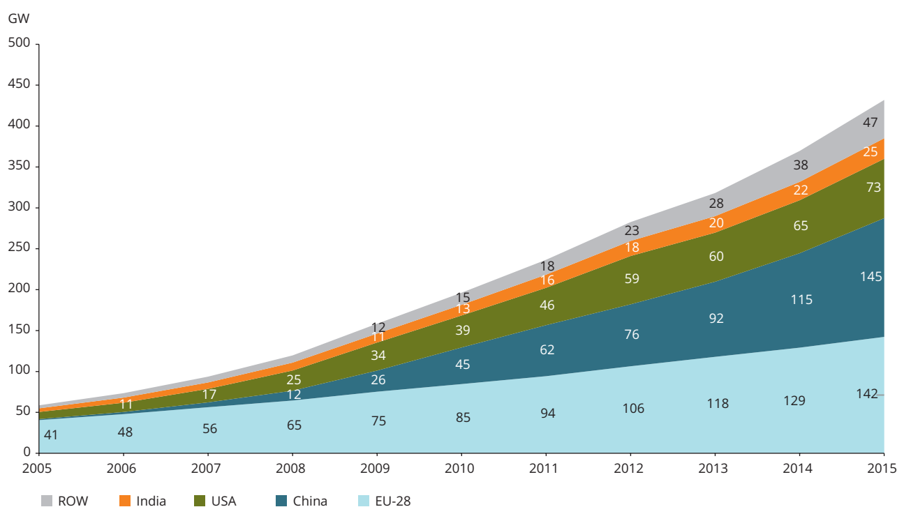
Figure 3.3 Growth in total wind power capacity (GW) in the EU-28, the top three non-EU countries and the rest of the world (ROW), 2005-2015
